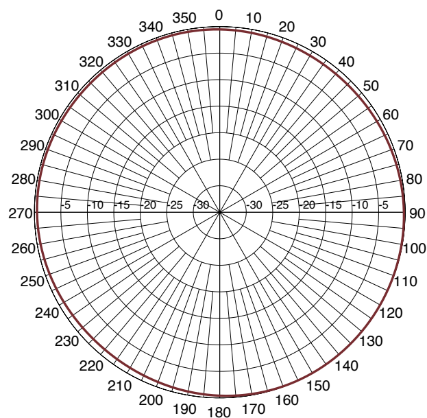
Azimuth Pattern at 5850MHz
