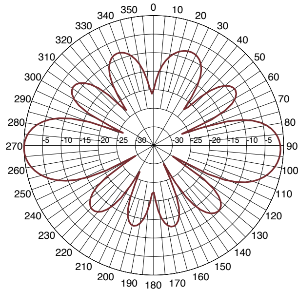
Elevation Pattern at 5150MHz
