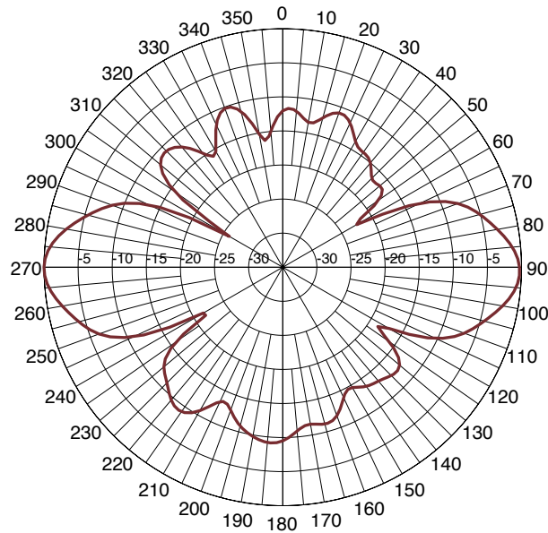
Elevation Pattern at 5850MHz
