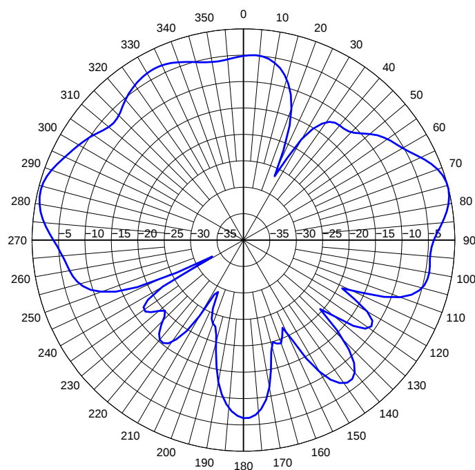
2500MHz Wi-Fi Phi 0 Elevation Pattern
