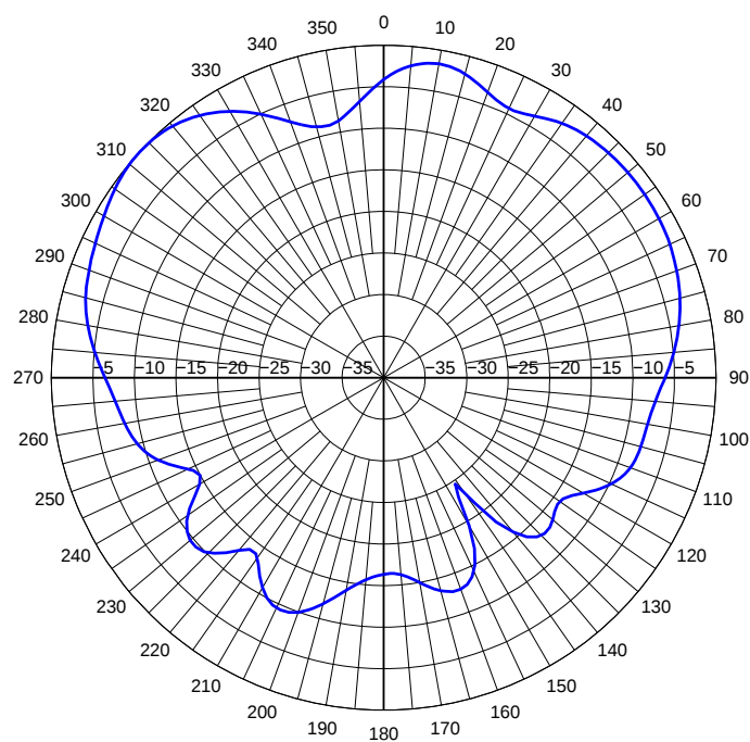
883MHz GSM 800 Phi 90 Elevation Pattern
