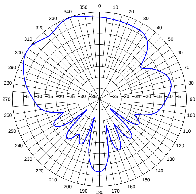
2010MHz GSM 1710 Phi 0 Elevation Pattern
