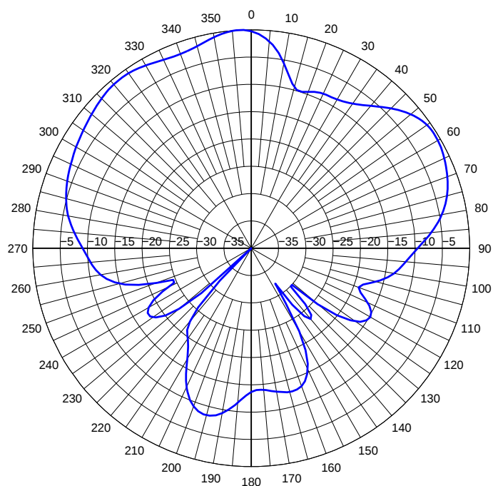
2010MHz GSM 1710 Phi 90 Elevation Pattern
