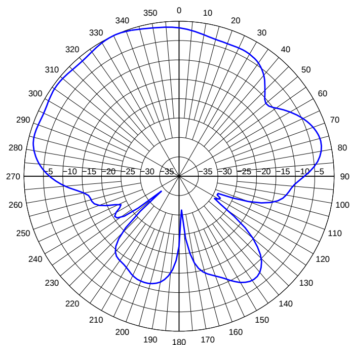
2500MHz Wi-Fi Phi 90 Elevation Pattern
