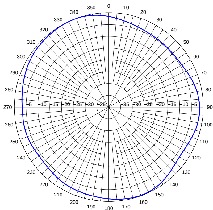
2500MHz Wi-Fi THETA 90 Azimuth Pattern
