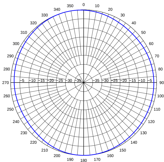
2010MHz GSM 1710 THETA 90 Azimuth Pattern
