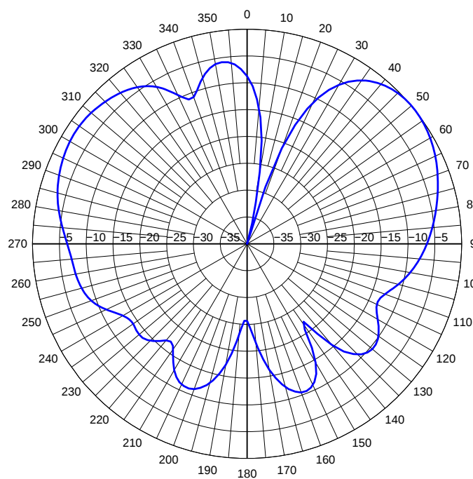
883MHz GSM 800 Phi 0 Elevation Pattern
