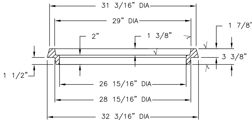
FRAME SECTION
