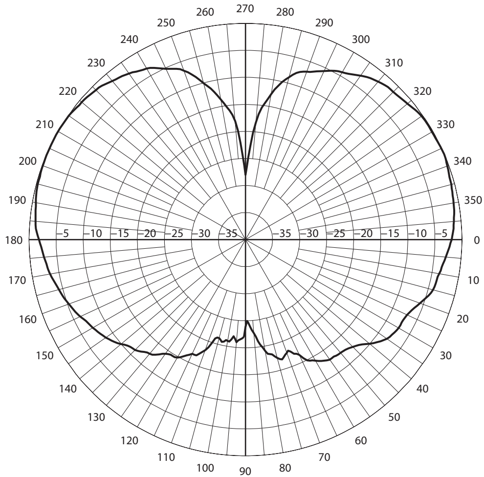
MLPV2400NGP Elevation Cut
