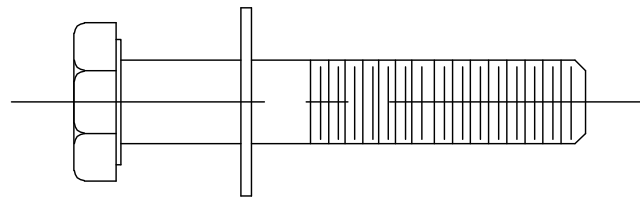
ILLUSTRATION #2 BOLT & WASHER ASSEMBLY
