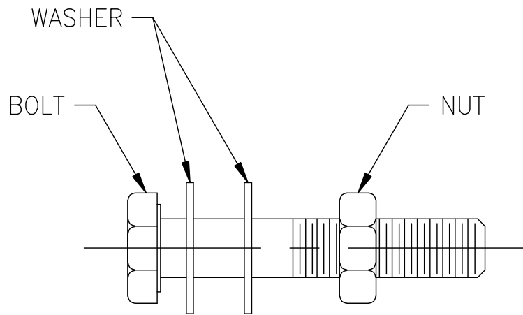
ILLUSTRATION #1 BOLT, WASHER & NUT ASSEMBLY
