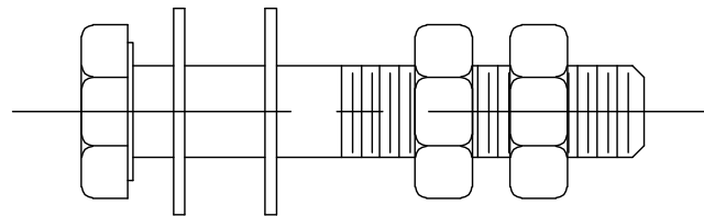
ILLUSTRATION #3 BOLT, WASHER & NUT ASSEMBLY
