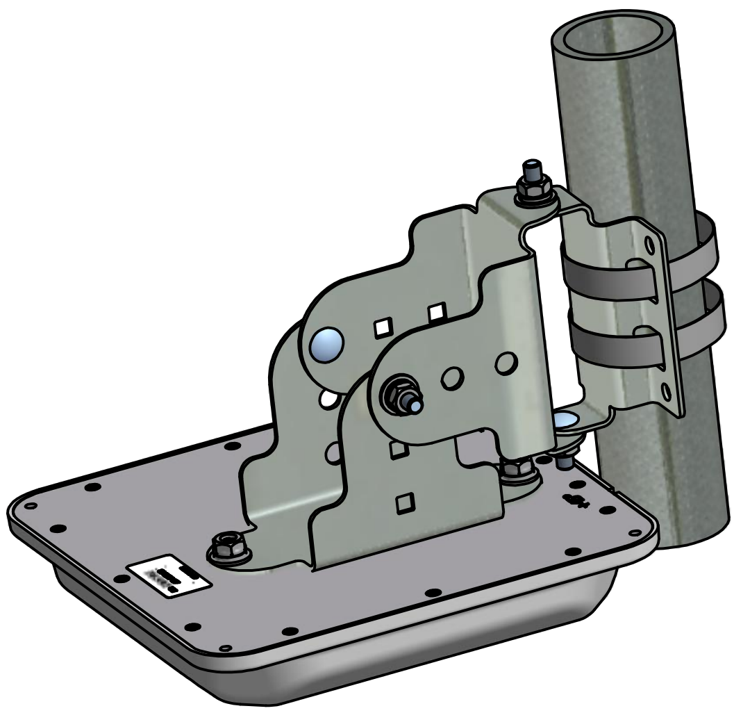
POLE MOUNTING
