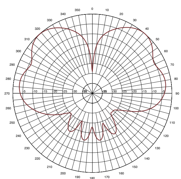
Elevation Pattern
