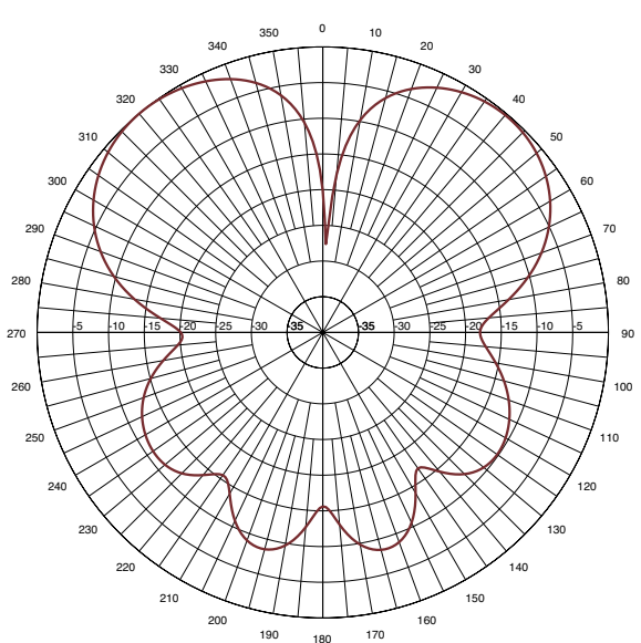
Elevation Pattern
