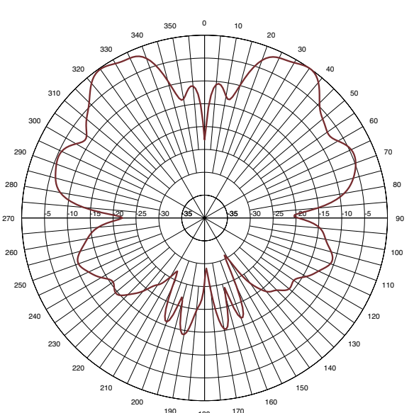
Elevation Pattern
