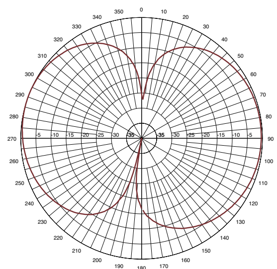
Elevation Pattern
