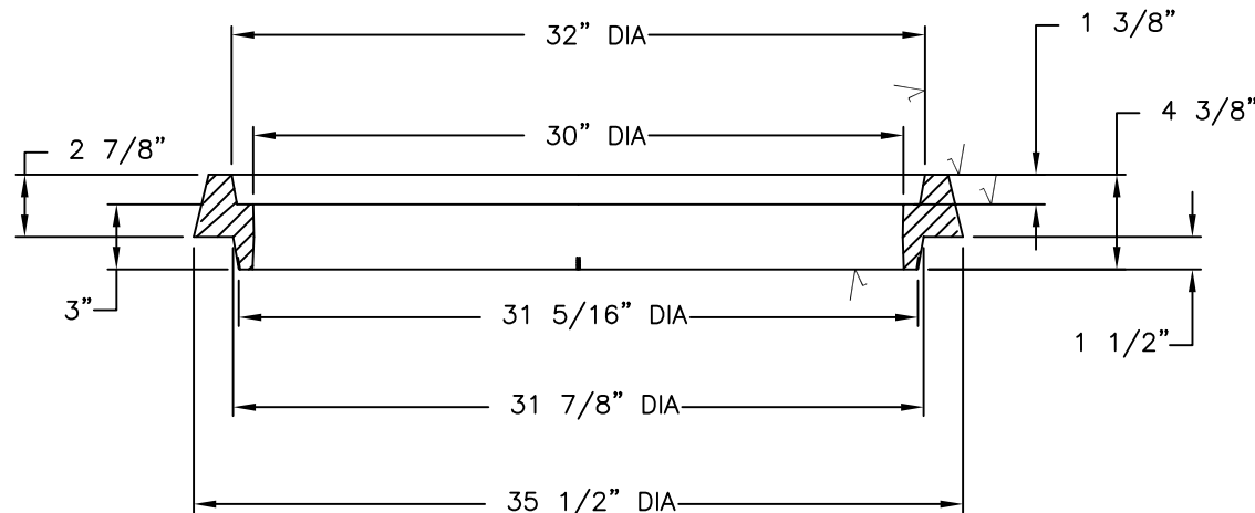
FRAME SECTION
