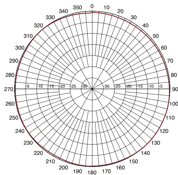
Azimuth Pattern at 3800MHz
