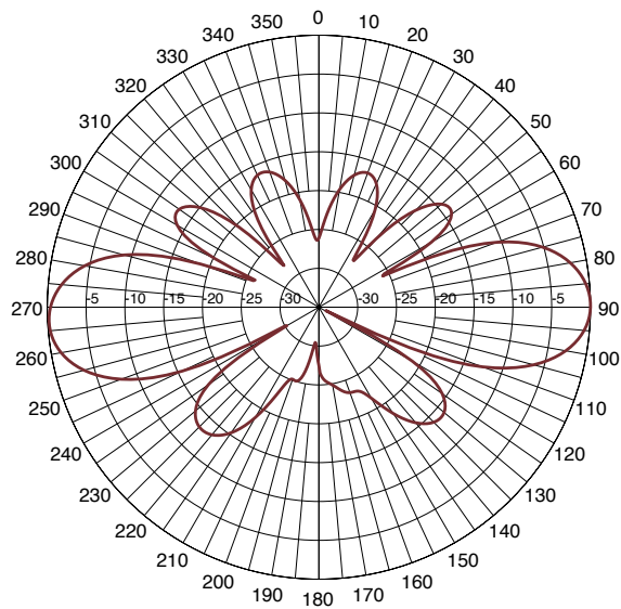
Elevation Pattern at 3600MHz
