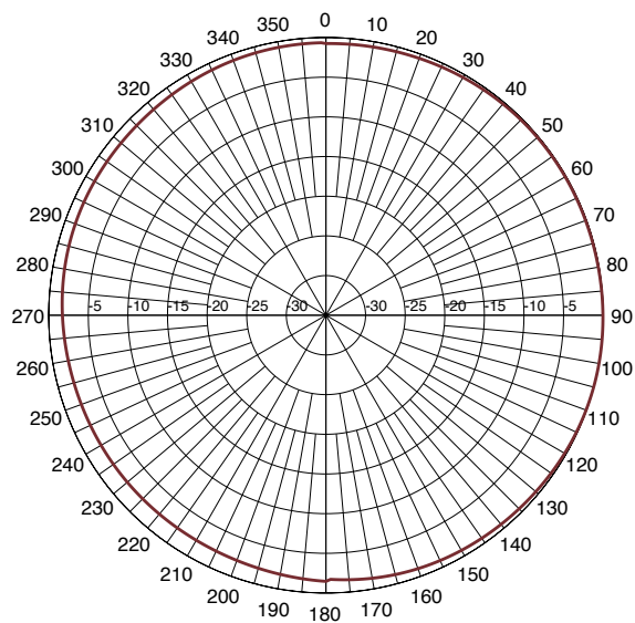
Azimuth Pattern at 3400MHz
