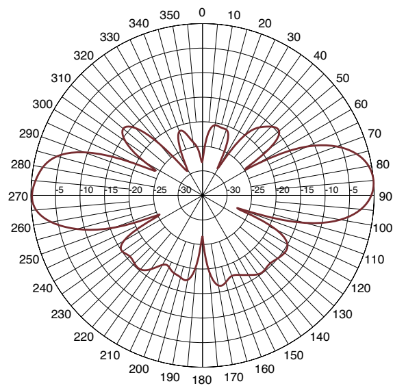
Elevation Pattern at 3800MHz
