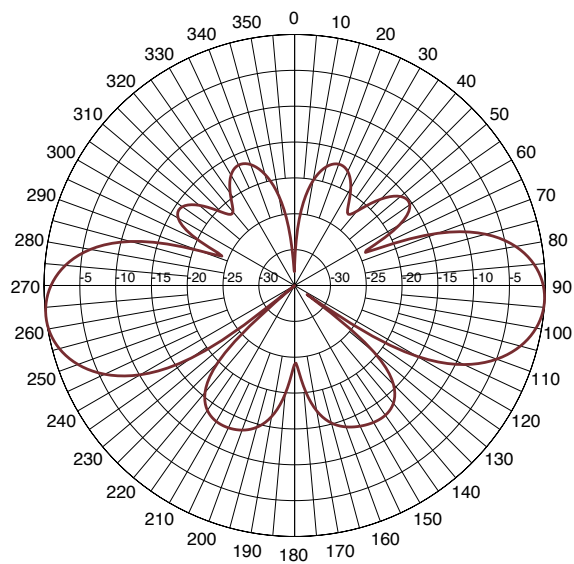
Elevation Pattern at 3400MHz
