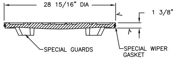
COVER SECTION
