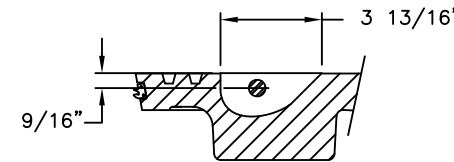
PICKBAR DETAIL
