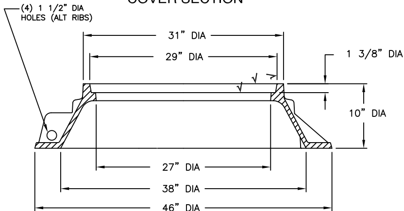
FRAME SECTION
